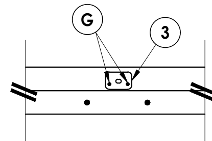
HINGE DETAIL
