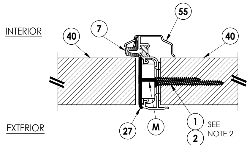
3 4 HORIZONTAL CROSS SECTION Outswing shown - inswing also approved
