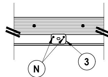
Inswing configuration
